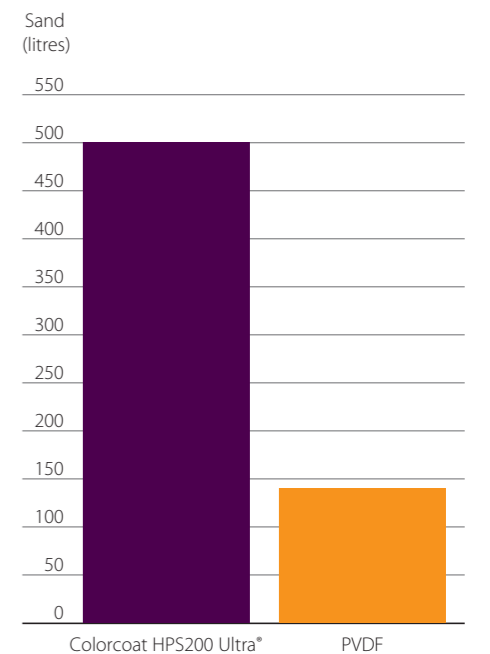
Figure 11. Abrasion resistance comparison (ASTM D968:2001)
